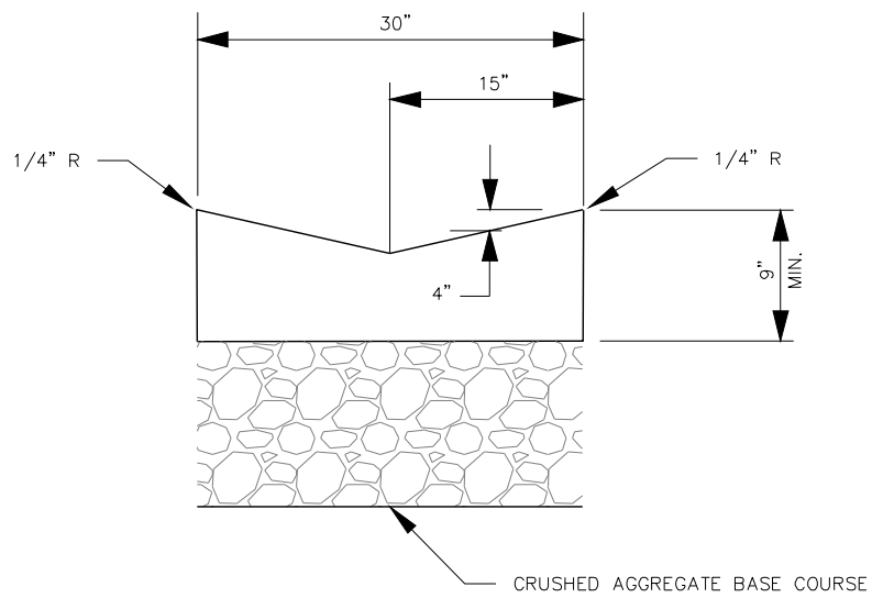
CONCRETE FLUME 30" (MIN. 3' LENGTH)
