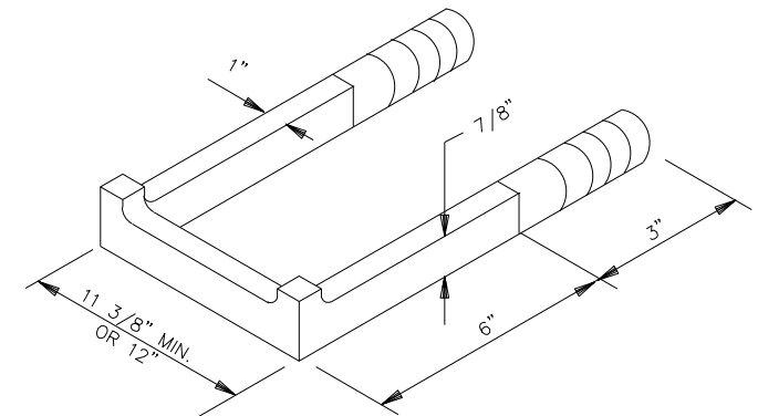
TYPICAL MANHOLE STEP
