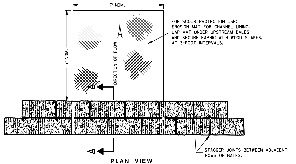
PLAN VIEW
