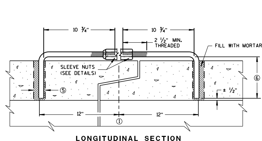
ADJUSTABLE TIE ROD (ALTERNATE NO. 3)
