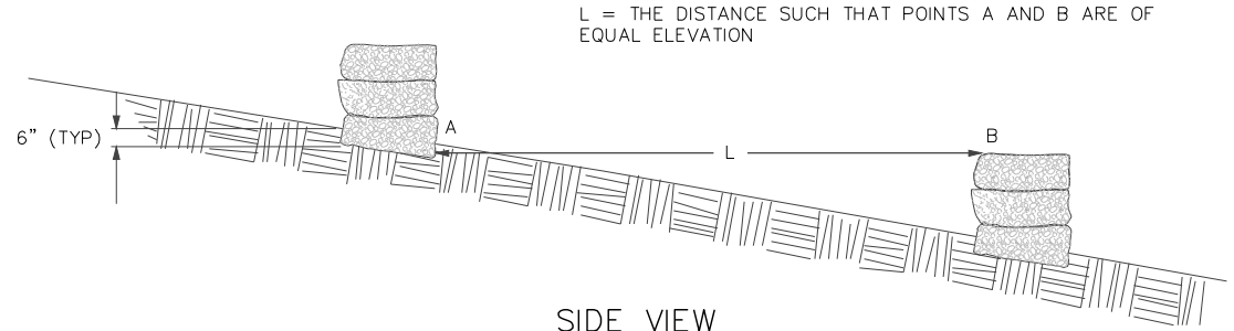
SIDE VIEW
