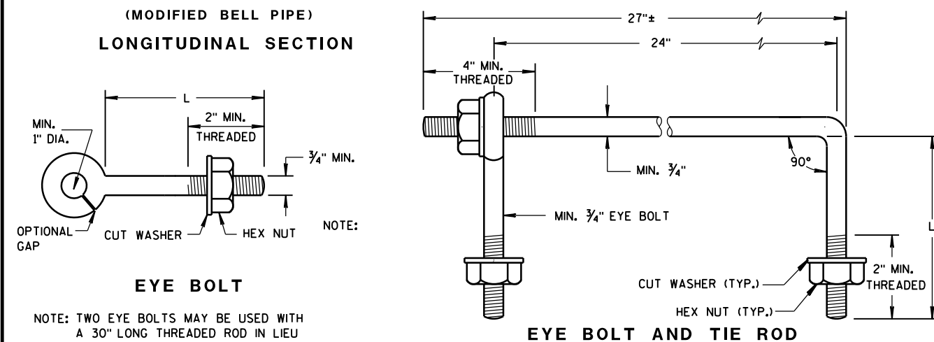
EYE BOLT AND TIE ROD ASSEMBLY (ALTERNATE NO. 2)
