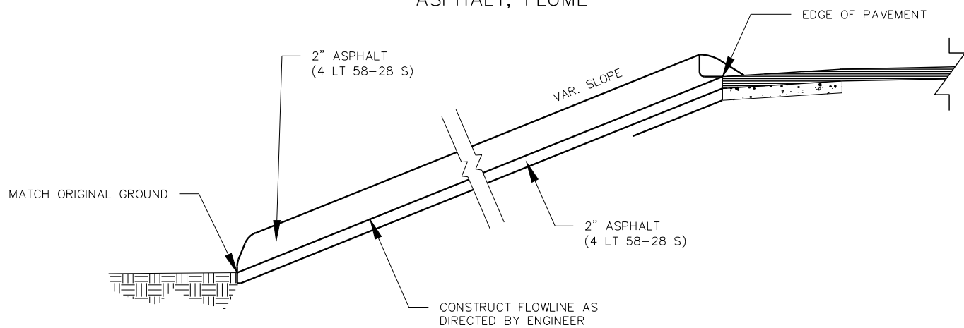
ASPHALT, FLUME
