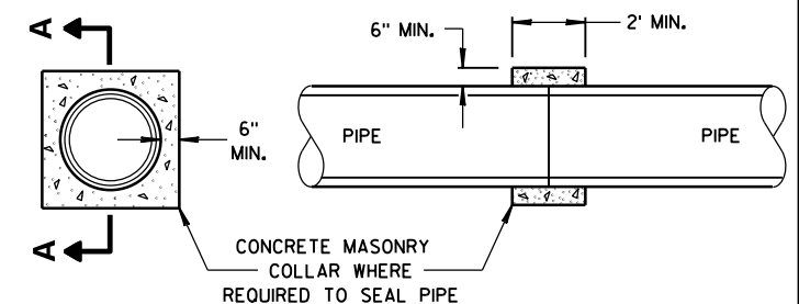
CONCRETE COLLAR DETAIL
