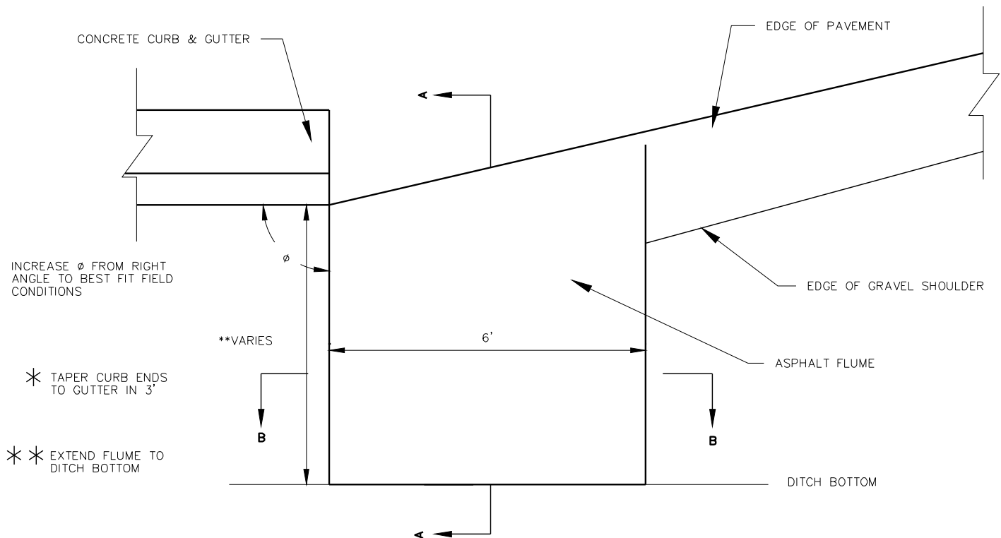
ASPHALT, FLUME
